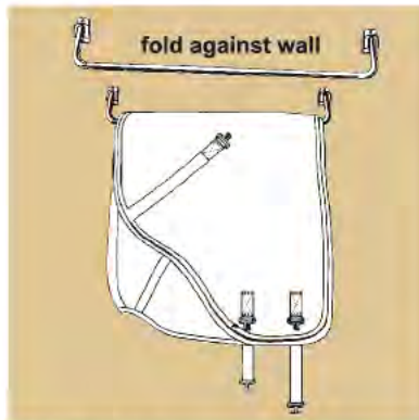
NO.2232 BLANKET BAR Collapsible bar designed to pull out for airing and storage of blankets coolers towels folds against wall of door when not in use, made of steel tubing and cast aluminium holder overall inside length is 91cm(36") 25/Box
