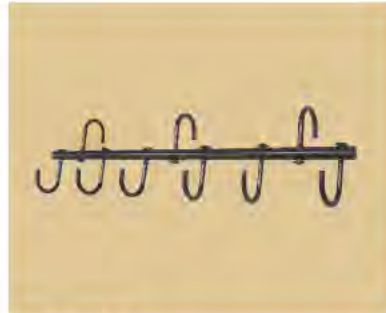
NO.2283 TACK BAR 6 hooks Made of tubular steel and chrome- plated with hooks that rotate and will hang of fence, wall raise etc. 69cm(27") long. Color:black(4) 50/Box
